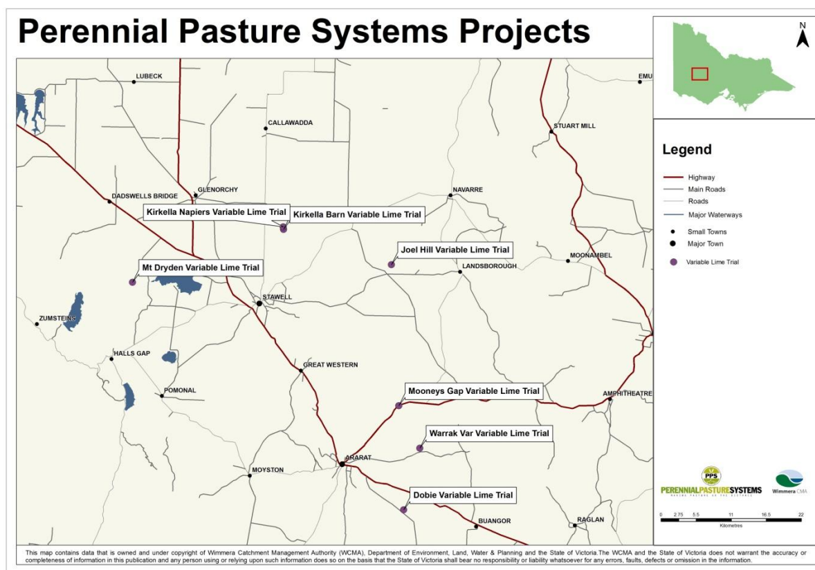
Figure 2; Map of pH testing sites
