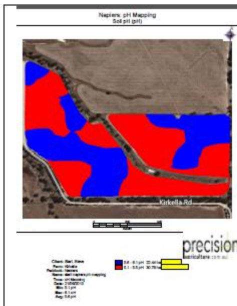
Figure 10 (left) schematic pH map; Kirkella – Napiers
