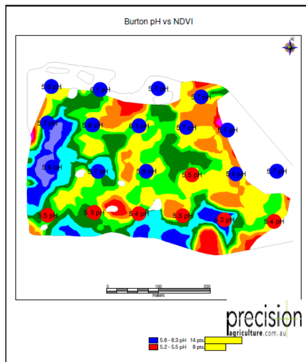
Figure 40: Redrawn pH Vs NDVI map
