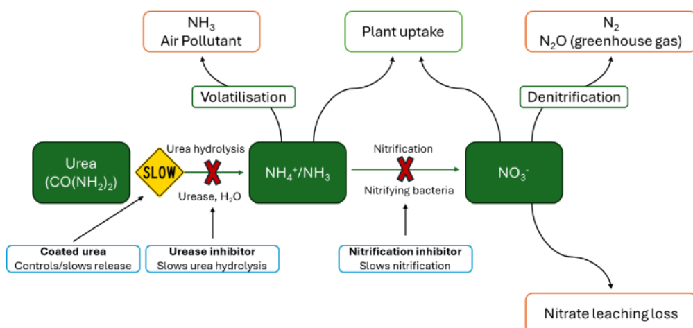
Figure 1. N pathways after application of urea and location of impact of the different EEFs and the impacted loss pathways. Adapted from Suter and Pandey, 2025.
