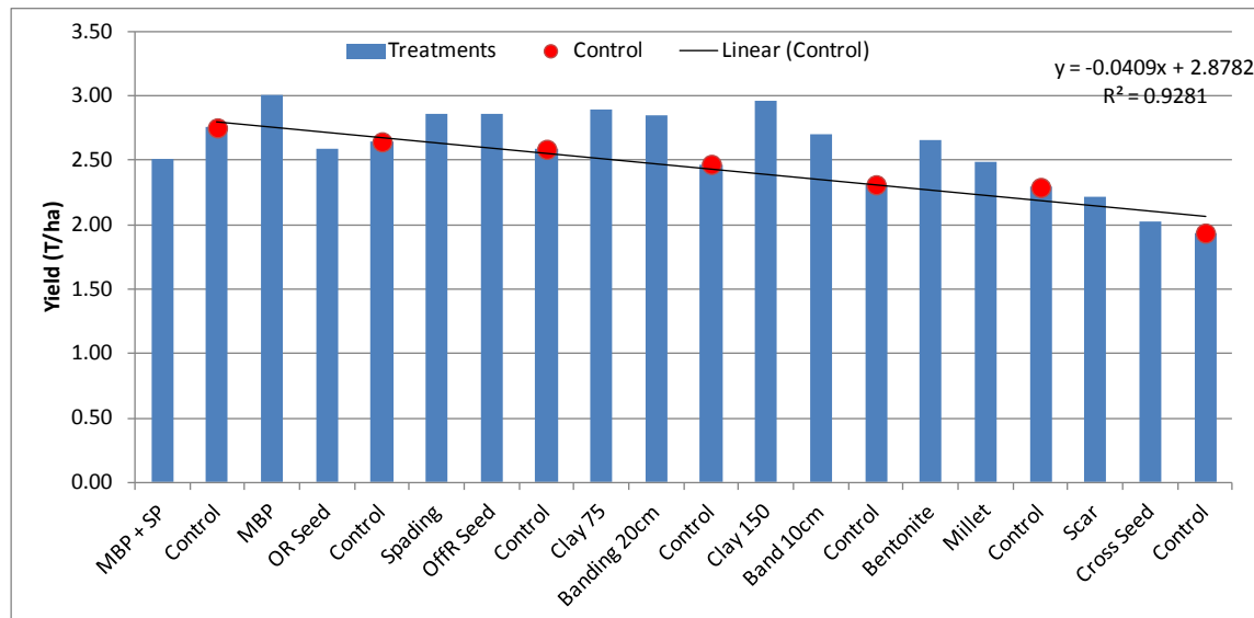
Figure 13. Yield of each plot and the spatial trend that exists at Lloyd Burrell.
