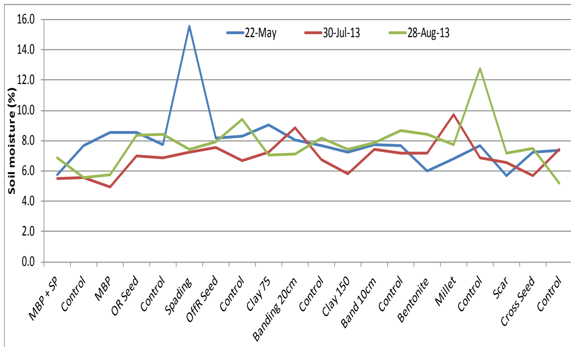
Figure 9. Soil moisture transect on three different dates at Lloyd Burrell.
