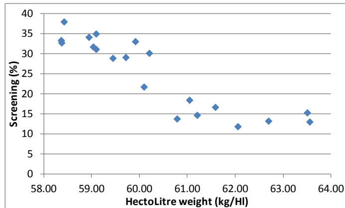
Figure 15 Relationship between the Hectolitre weight and the screenings at Lloyd Burrell
